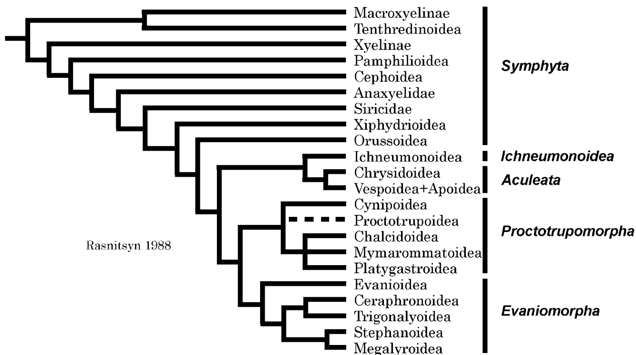
FIGURE 4. Simplified interpretation of the phylogenetic tree from Rasnitsyn (1988). Dashed branch indicates Proctotrupoidea as a paraphyletic grade.
