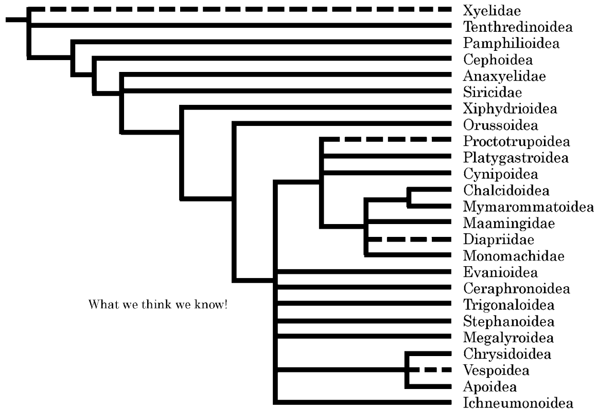
FIGURE 13. Phylogenetic tree summarizing relationships that are reasonably well corroborated by published analyses. Dashed lines indicate taxa of questionable monophyly.
