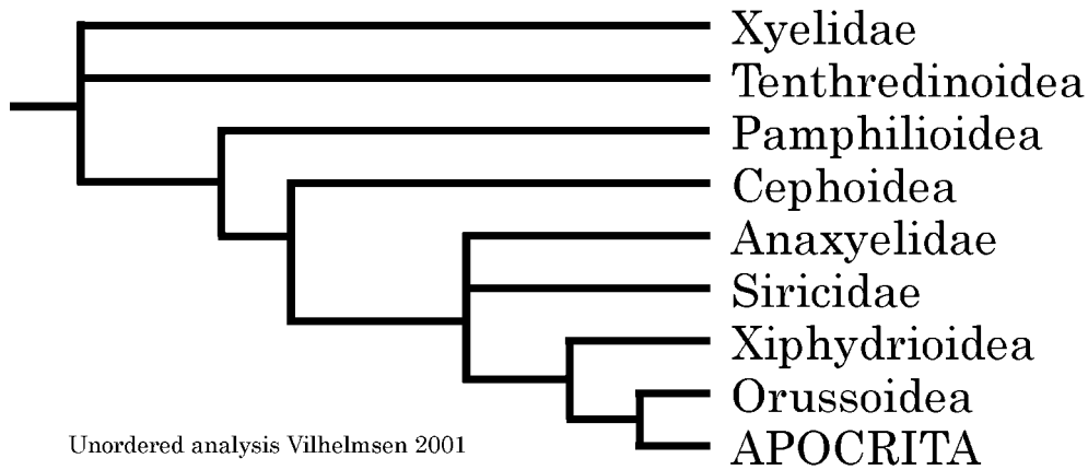
FIGURE 8. Strict consensus tree of basal hymenopteran taxa based on unweighted parsimony analysis of unordered morphological data, simplified from Vilhelmsen (2001).
