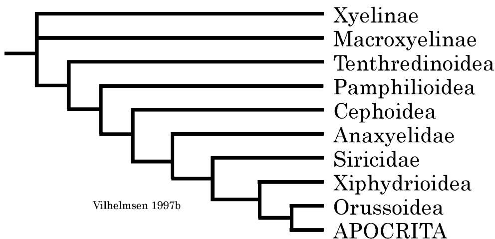
FIGURE 7. Strict consensus tree of basal hymenopteran taxa based on unweighted parsimony analysis of unordered morphological data, simplified from Vilhelmsen (1997b).
