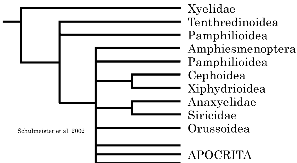
FIGURE 9. Summary tree of basal hymenopteran taxa based on nuclear rDNA genes 18S and 28S and mitochondrial genes 16S rDNA and CO1, simplified from Schulmeister et al. (2002).
