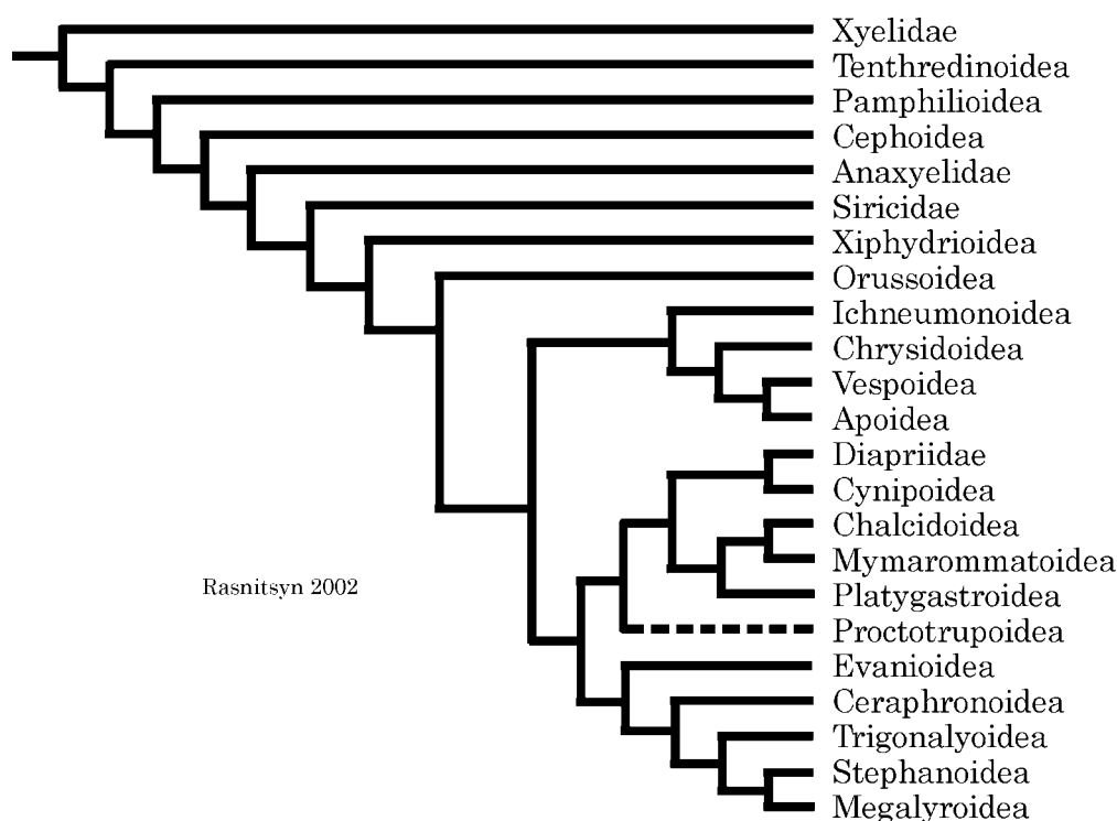
FIGURE 5. Simplified interpretation of Rasnitsyn's most recent hypothesis inferred from Rasnitsyn (2002) and Rasnitsyn et al. (2004).
