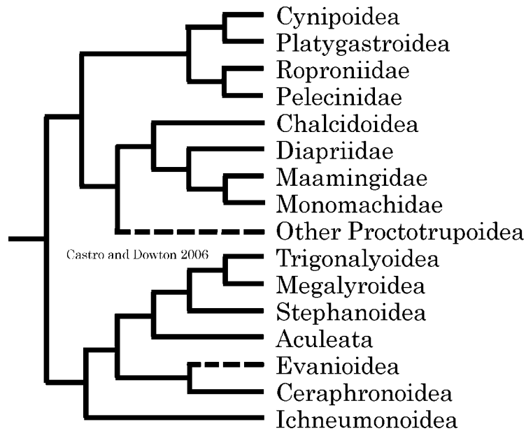
FIGURE 12. Strict consensus tree of apocritan taxa based on mitochondrial genes 16S rDNA and CO1, and nuclear genes 28S rDNA and 18S rDNA, simplified from Castro and Downton (2006). Dashed lines indicate taxa that may be paraphyletic.
