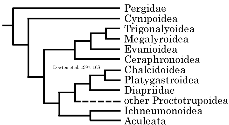
FIGURE 10. Strict consensus tree of apocritan taxa based on mitochondrial gene 16S rDNA, simplified from Dowton et al. (1997). Dashed line indicates a paraphyletic Proctotrupeoidea.
