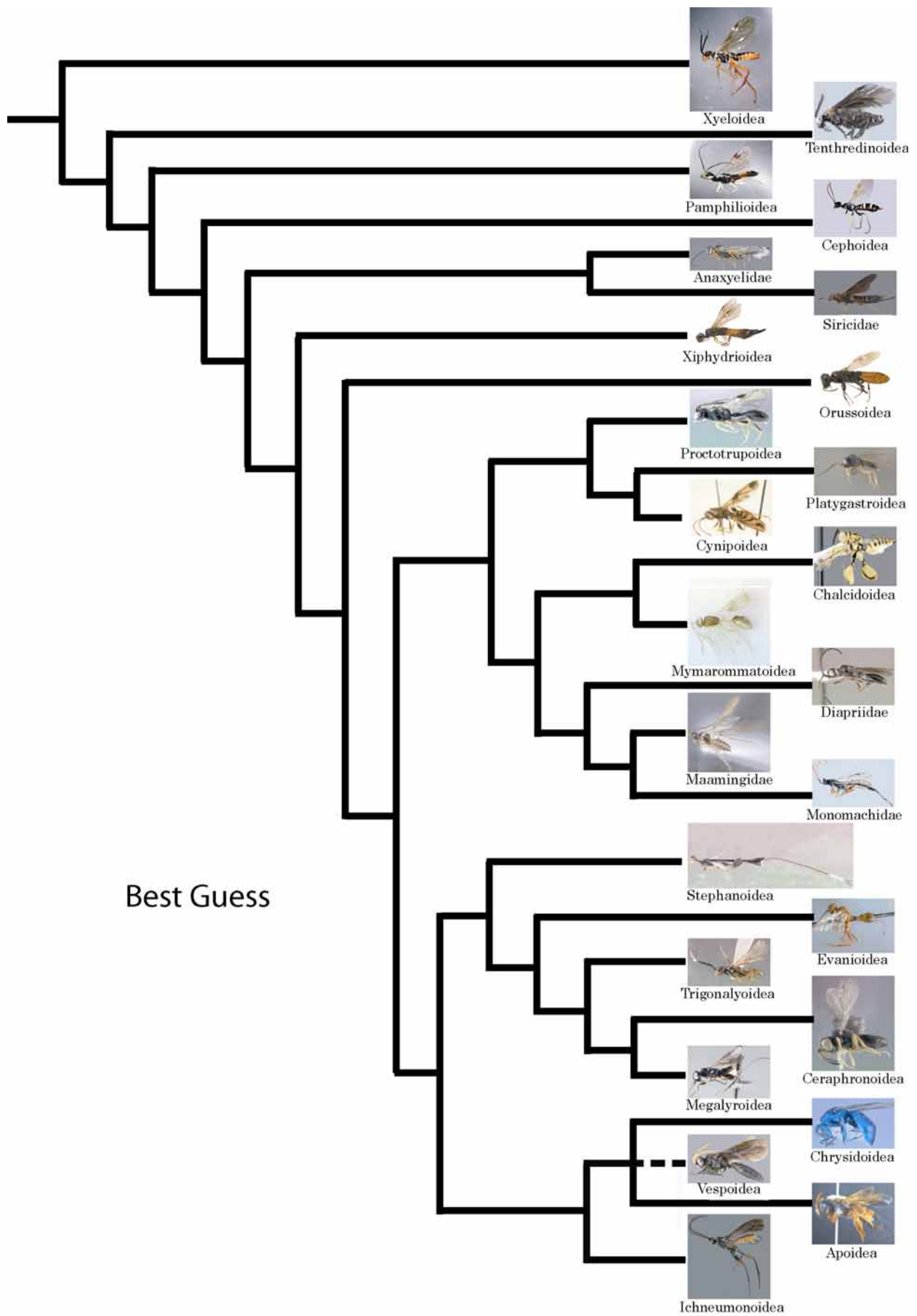
FIGURE 14. Intuitive phylogenetic tree based on relationships that have some support in published analyses. Click on thumbnail images to link to larger images.
