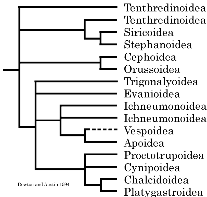
FIGURE 6. Strict consensus tree of hymenopteran relationships based on unweighted parsimony analysis of 16S data, simplified from Dowton and Austin (1994).
