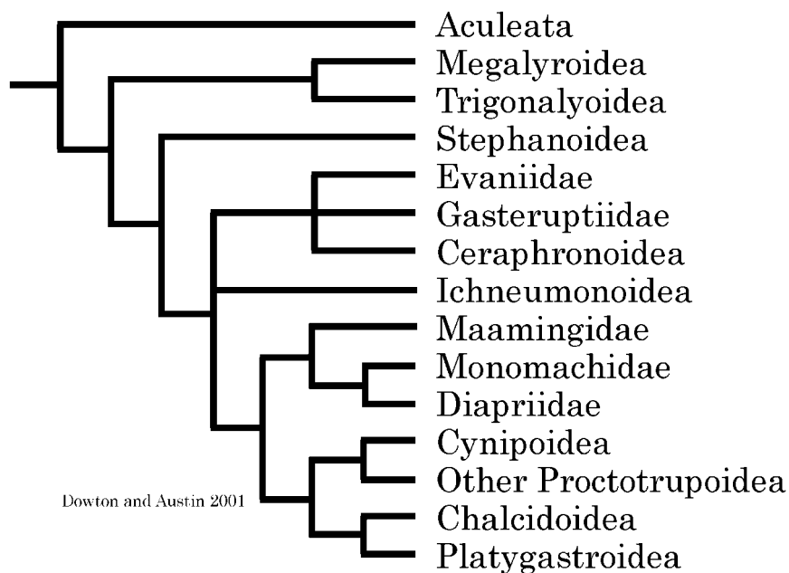
FIGURE 11. Strict consensus tree of apocritan taxa based on mitochondrial genes 16S rDNA and CO1, and nuclear gene 28S rDNA, simplified from Dowton and Austin (2001).
